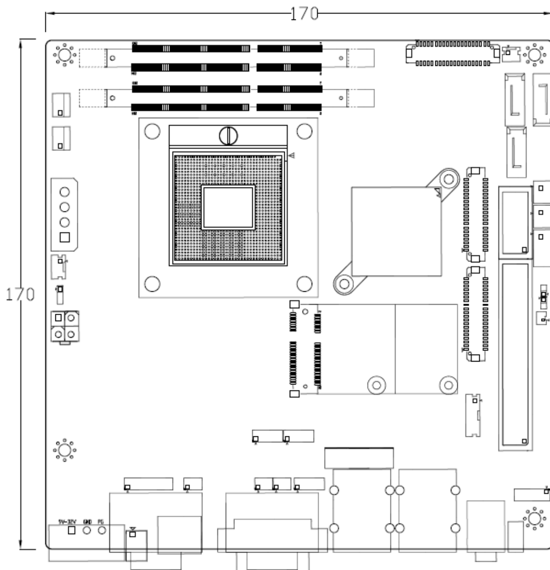
Figure 2.1: Mainboard Dimensions
