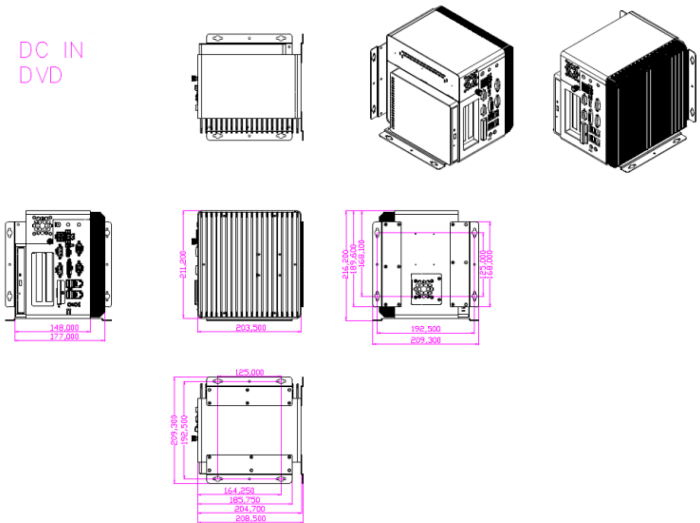
Figure 1.1: Dimensions of the NV-2695A
